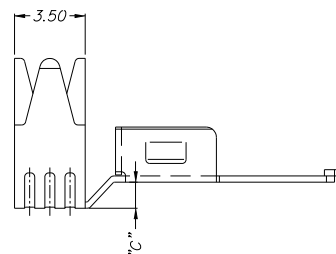
FRONT SHELL
