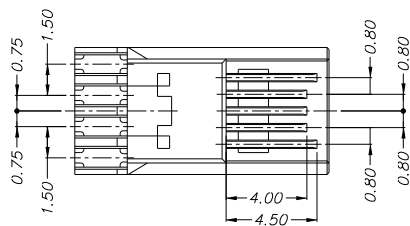
HOUSING+TERMINAL
