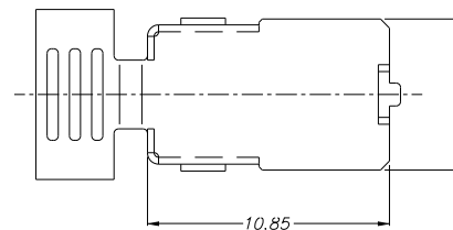
REAR SHELL
